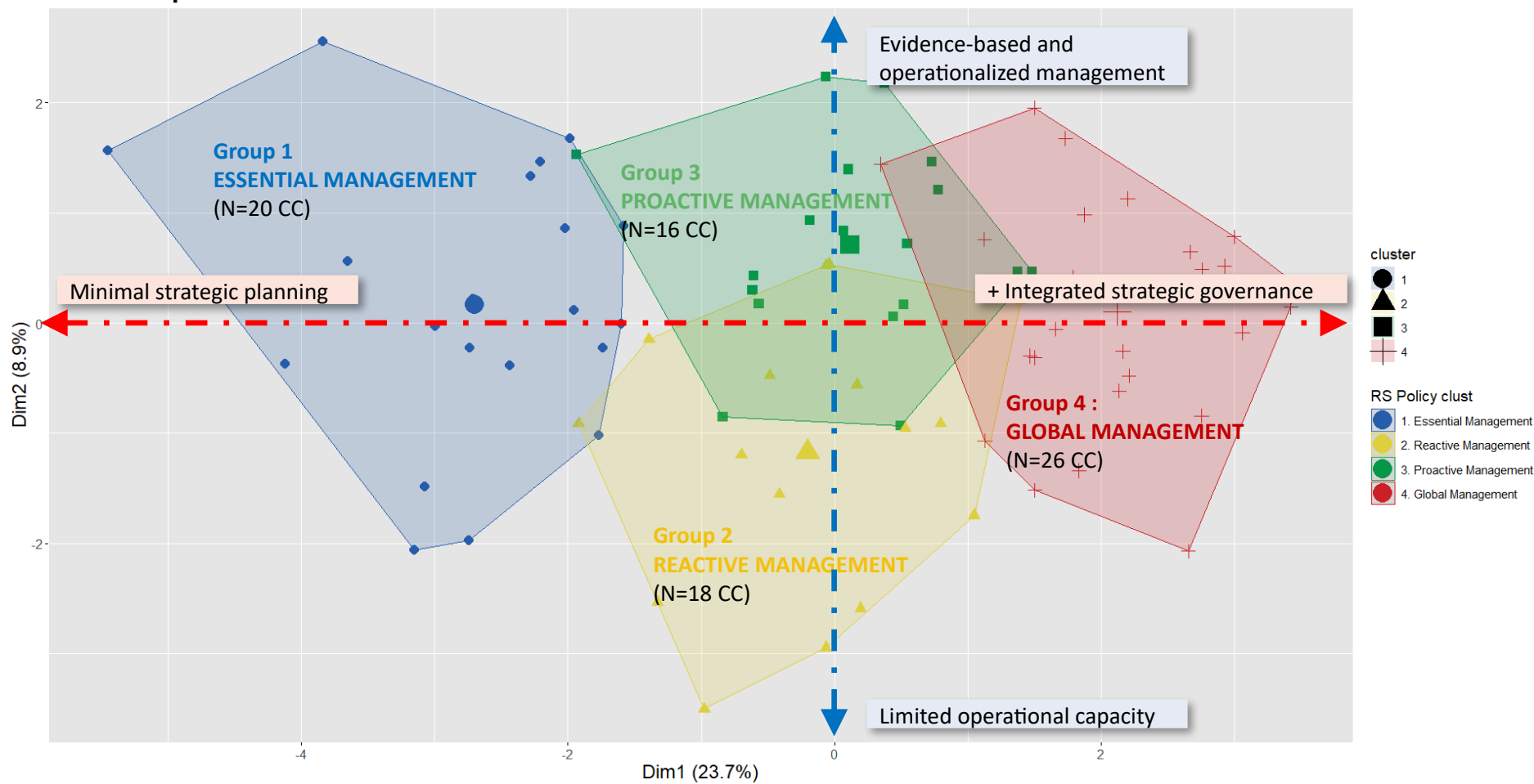
Factor map FAMD
